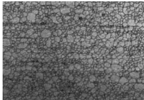
Electrolytic etched Stainless Steel
